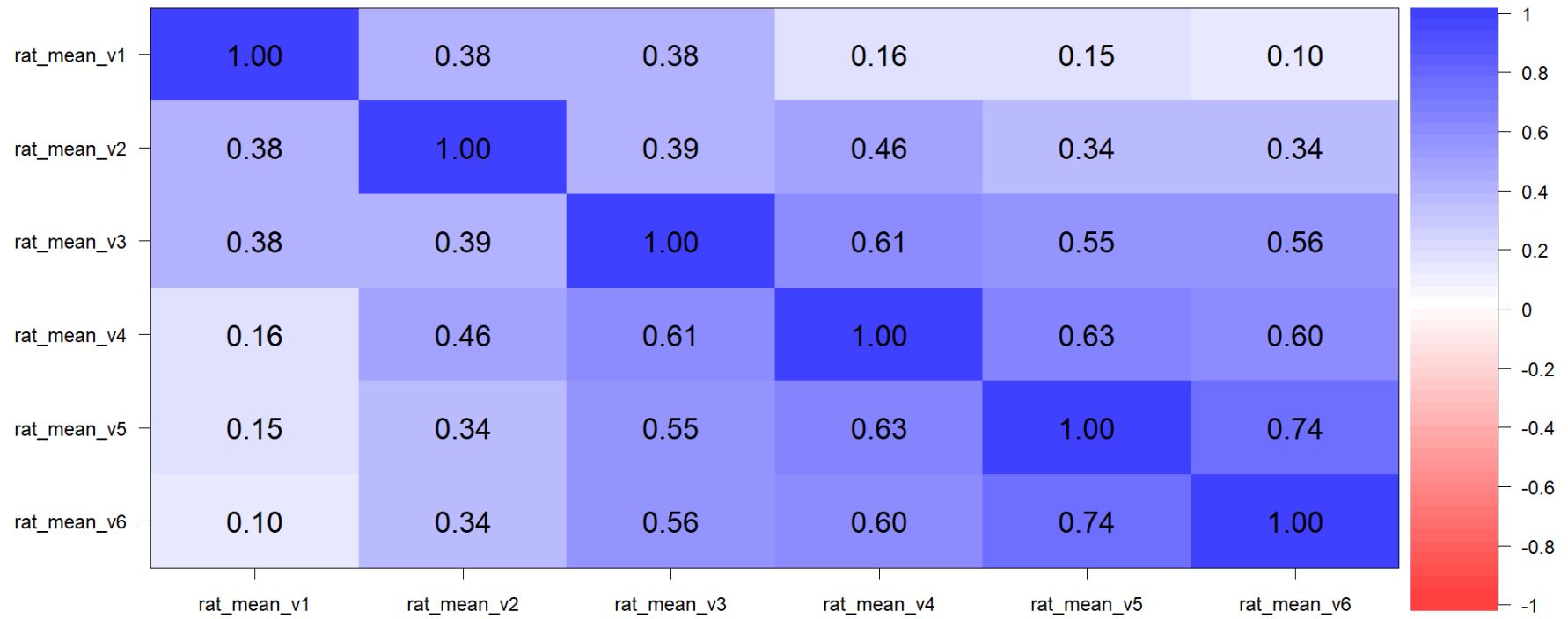
Manifest Correlations
